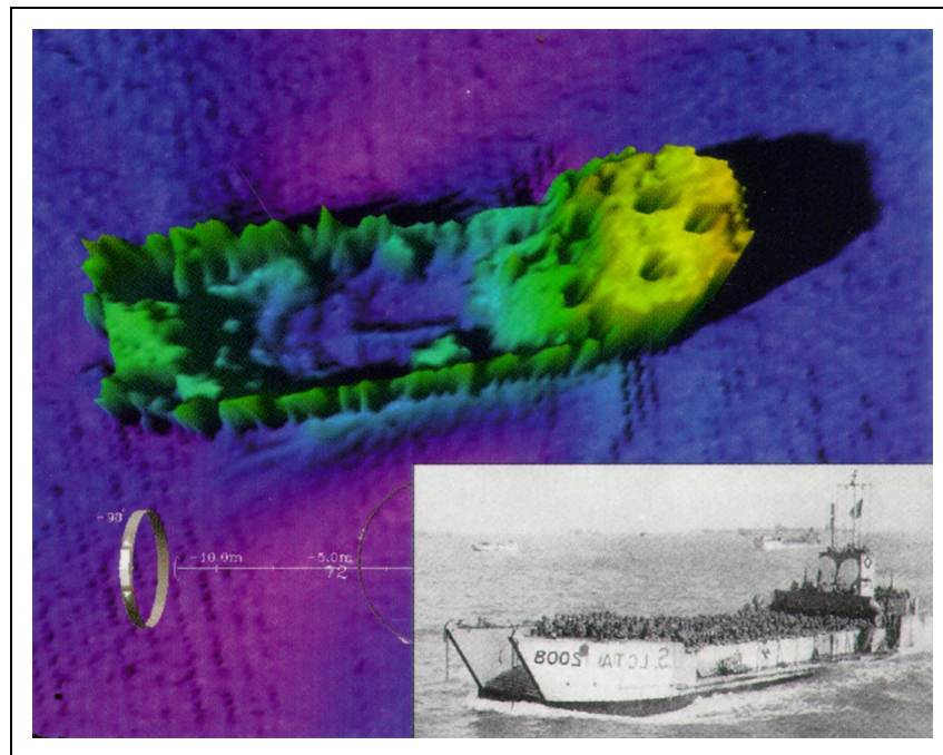
FIGURE 5. Reson Sea Bat 8125 image of a World War II LCT sunk off Omaha Beach, Normandy during the D-Day Landing (Image courtesy of Reson and the Naval Historical Center).
