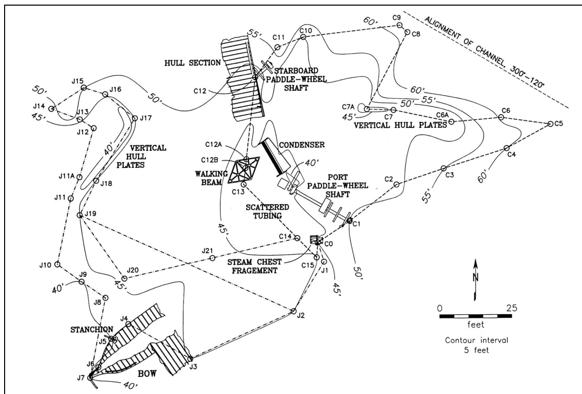
FIGURE 7. Plan of the surviving remains of steamship Mary sunk adjacent to the Aransas Pass, Texas navigation channel (Image courtesy of Coastal Environments, Inc., 1977).
