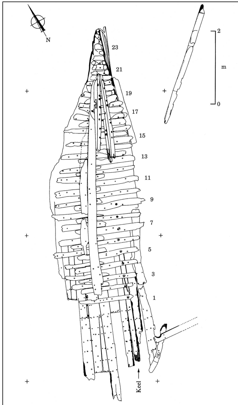
FIGURE 6. Plan of the surviving remains of the mid-fifteenth century shipwreck discovered during dredging of the Ria de Aveiro, Portugal (Site plan courtesy of Miguel Aleluia).
