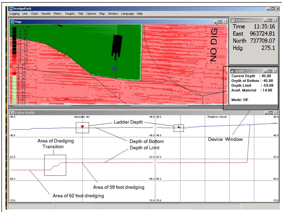
FIGURE 21. A screen from the software DREDGEPACK. The dredge is positioned near a transition point in the dredging project. Several items have been identified in the image. The device window shows the Current Depth, Depth of Bottom, Depth Limit, Depth of Available Material and the Current Mode if there is a violation or not. In the Map window a color filled matrix is displayed showing the current difference values for each cell. The color settings are set from -1 to 10. These values represent the difference between how much material is in the cell against the theoretical limit within that cell. If the operator violates the limit an alarm is sounded and displayed on the Survey screen. As the ladder transitions between depth limits, no operator interaction is required to reconfigure the software. Because the difference and the limit depth have been set, each cell acts independently of the others creating a seamless user interface. (Illustration courtesy of Coastal Oceanographics, Middlefield, Connecticut).
