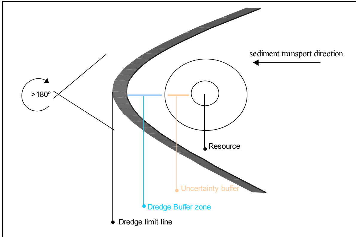
FIGURE 20. Guideline for dredging around a resource to prevent development of pedestals.
