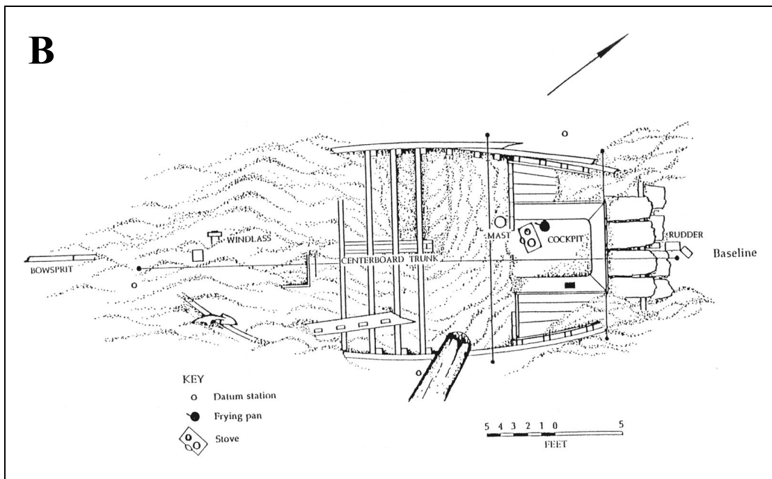
FIGURE 9. Illustration of the remains of the mid-nineteenth century Hilton Wreck schooner (A) prior to damage by dragging a cable across the hull and (B) after dragging a cable across the hull (Watts, 1994).
