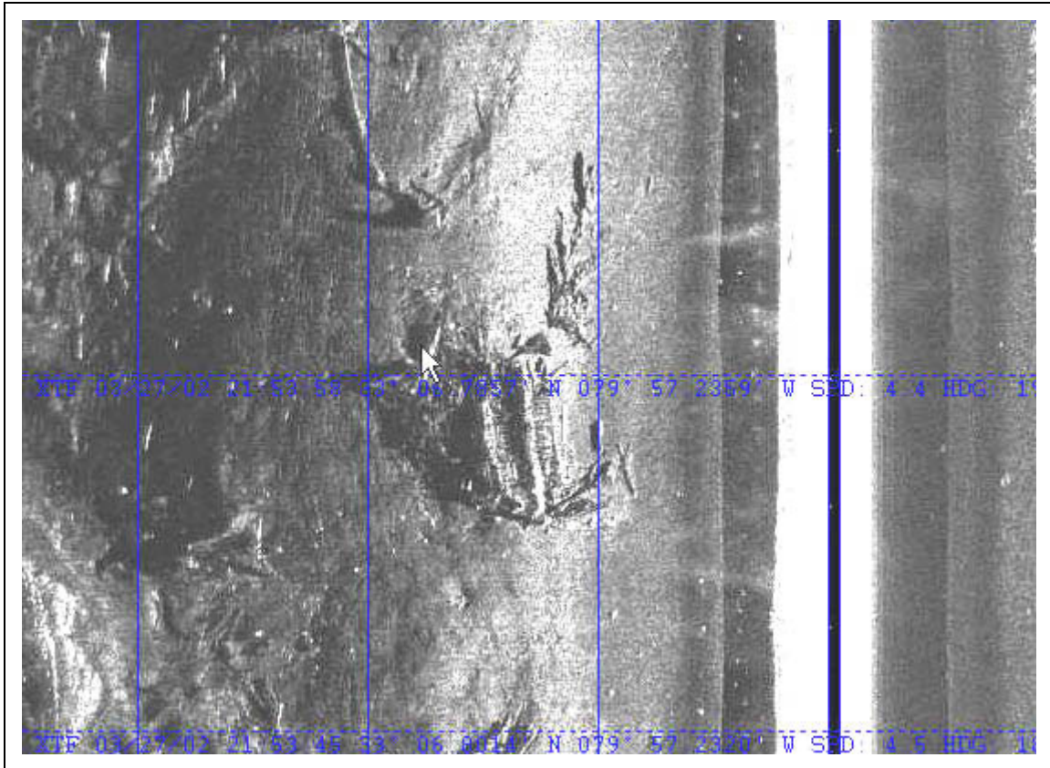
FIGURE 15. High-resolution Klein 500 kHz side scan sonar image of the remains of the Mepkin Abby vessel sunk in the Cooper River near Charleston, South Carolina (Image courtesy of Ralph Wilbanks, Diversified Wilbanks, Inc.).
