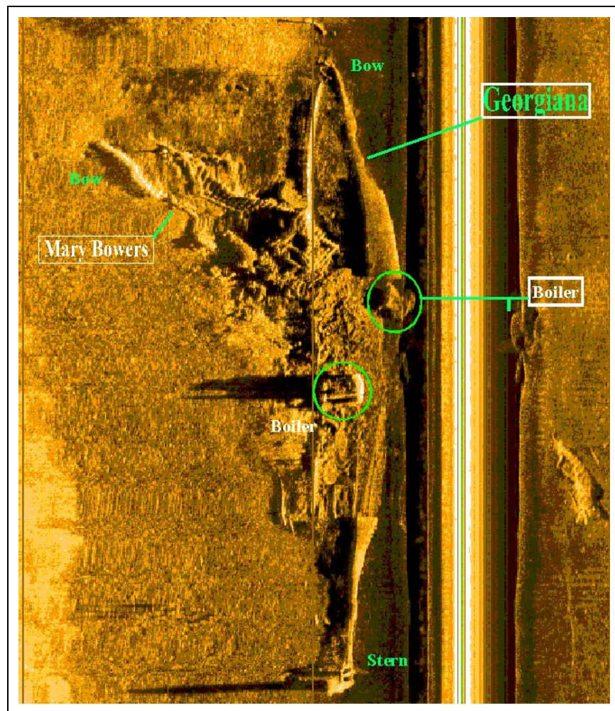
FIGURE 3. High-resolution Klein 500 kHz side scan sonar image of the Civil War blockade runners Georgiana and Mary Bowers sunk off Charleston, South Carolina (Image courtesy of Ralph Wilbanks, Diversified Wilbanks, Inc.).
