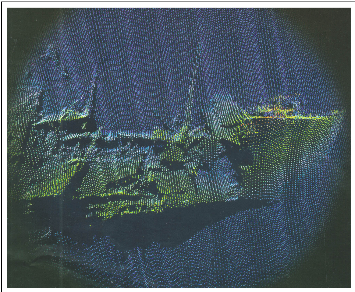
FIGURE 12. Reson Sea Bat 8125 data point image of the Susan B Anthony sunk off Omaha Beach, Normandy during the D-Day Landing (Image courtesy of Reson and the Naval Historical Center).
