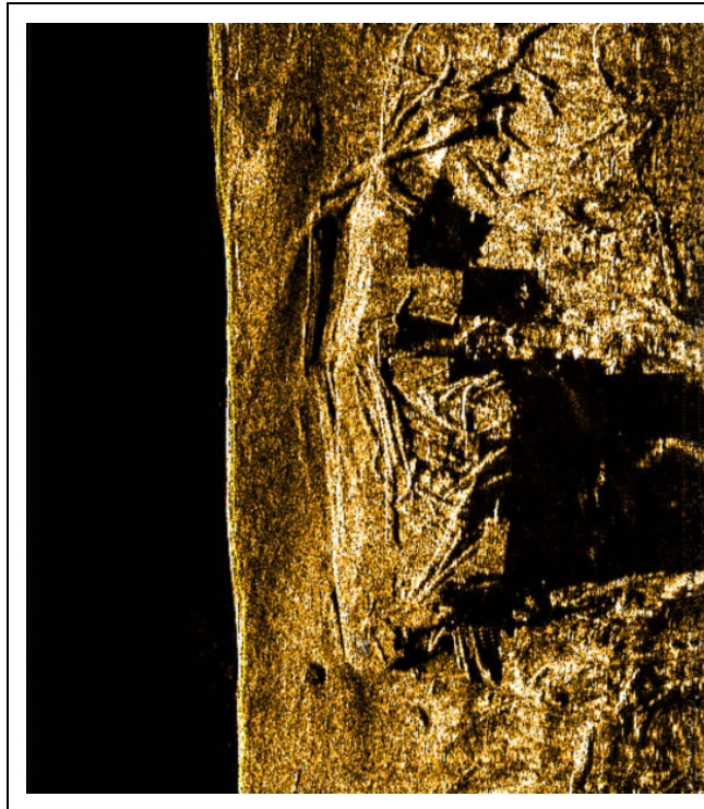
FIGURE 11. Klein 3000 image of the remains of the ironclad CSS Georgia recorded at a distance of 75 m (A) and at a distance of 25 m (B) (Image courtesy of Georgia Department of Natural Resources).
