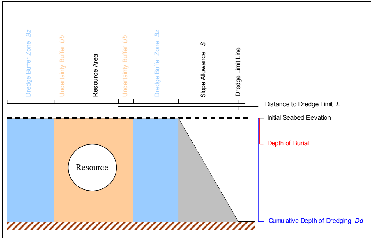
FIGURE 18. Diagram showing the parameters for calculating site-specific buffer zones.
