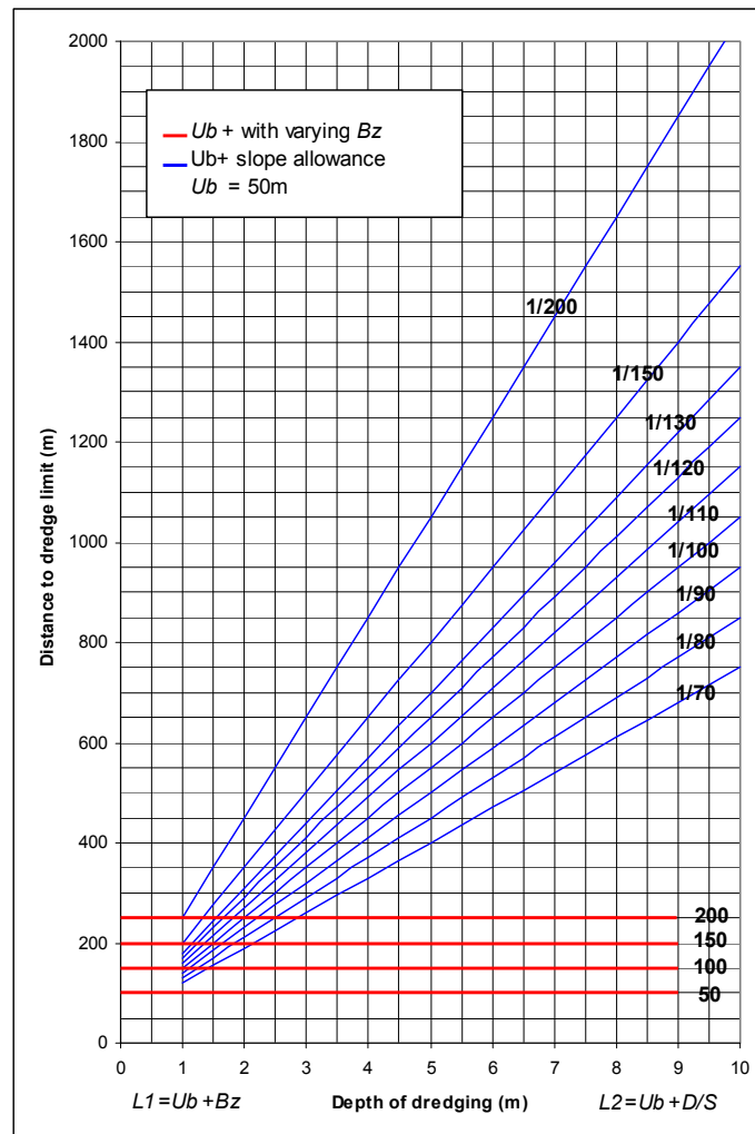
FIGURE 19. Distance from edge of resource to dredge limit line with different slope conditions.
