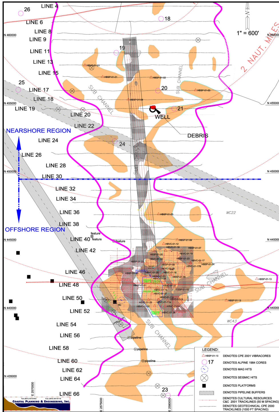
FIGURE 2. Map of the Holly Beach “fluvial system” at a 300 m spacing between tracklines for the geotechnical investigation and the higher density mapping (50 m) of the fluvial channels for cultural resources (in the south) in a proposed borrow area and overburden disposal site off Louisiana. With the more intensive survey, it was possible to delineate relic landforms with much greater detail, as seen in the southern area (Image courtesy of Coastal Planning & Engineering, Inc.).
