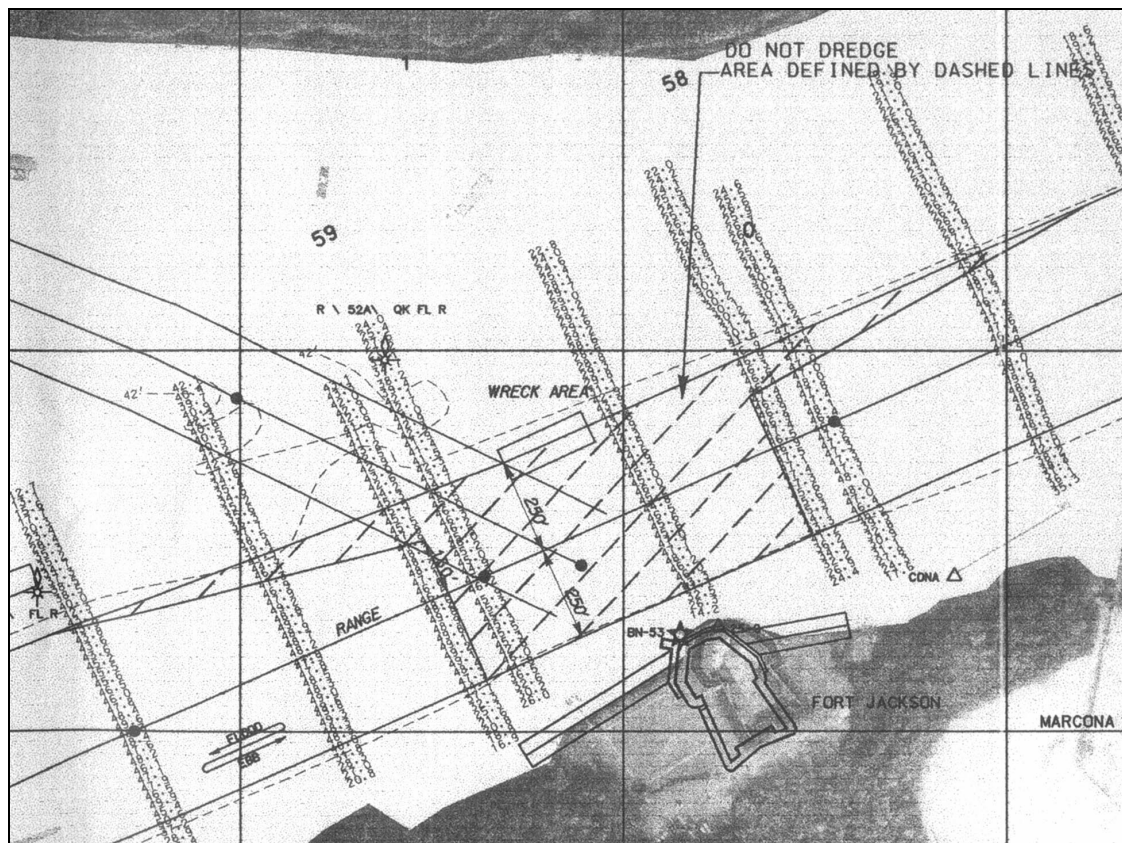
FIGURE 17. Buffer zone established by the Savannah District USACE to protect the remains of the Confederate ironclad CSS Georgia . (Illustration courtesy of the USACE Savannah District).
