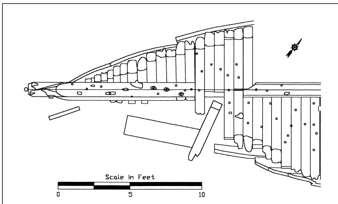
FIGURE 8. Plan of the bow of the ironclad CSS North Carolina illustrating the damage done by anchoring in the wreck (Image courtesy of Tidewater Atlantic Research, Inc.).
