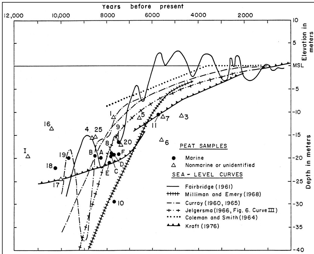
FIGURE 1. Sea-level curve showing the rapid rise in sea level at the end of the Late Wisconsinian glaciation, starting about 10,000 years ago (Murphy, 1990).
