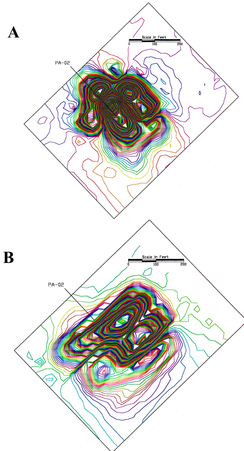
FIGURE 16. Magnetic signature of the Civil War ironclad USS Patapsco sunk in Charleston Harbor, South Carolina contoured from data recorded on 75-ft line spacing (A) and 150 ft line spacing (B) (Image courtesy of Tidewater Atlantic Research, Inc.).
