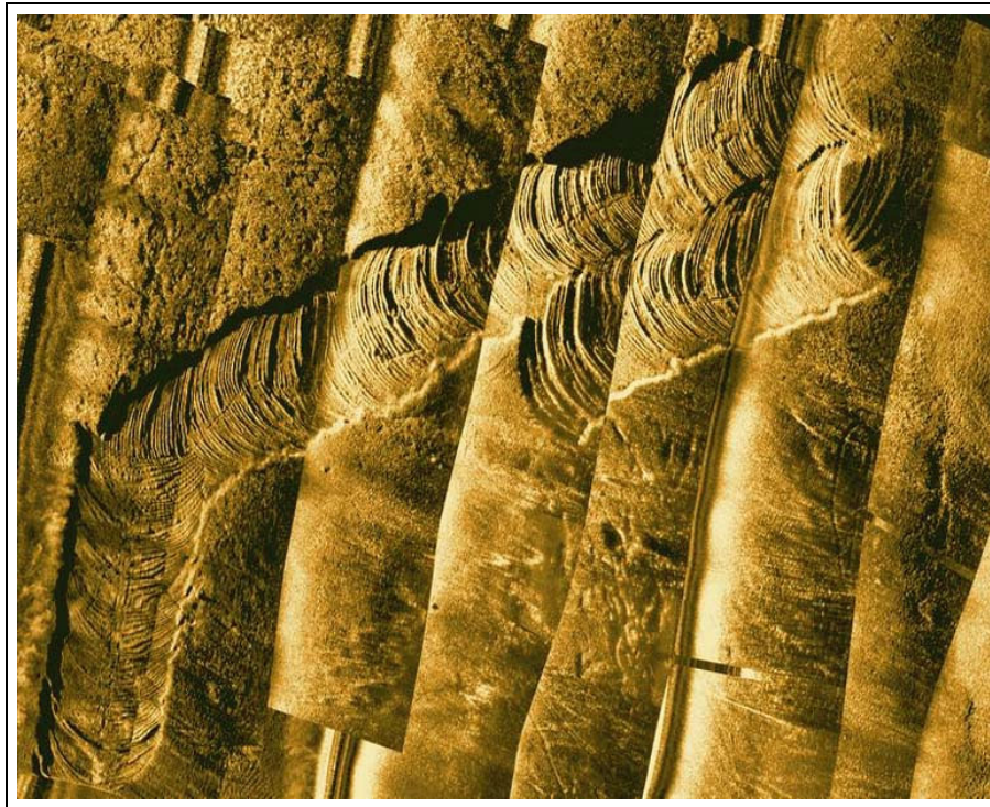
FIGURE 4. Mosaic of dredging scars compiled from high-resolution 600 kHz sonar images (Image courtesy of Marine Sonic Technology and Ocean Star Systems).
