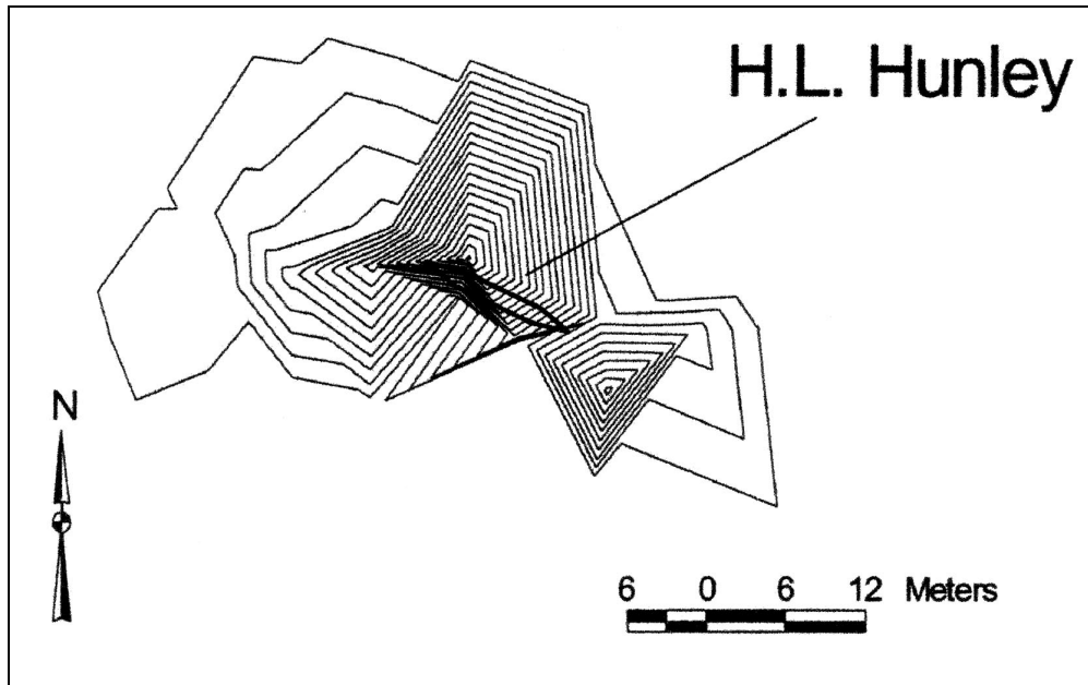
FIGURE 13. Contoured magnetic signature of the Confederate submarine CSS Hunley (Image courtesy of Reson and the Naval Historical Center).
