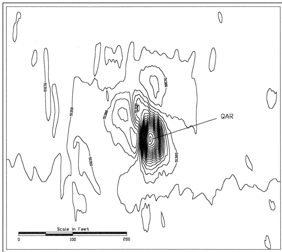
FIGURE 14. Contoured magnetic signature of the Eighteenth century shipwreck identified as the Queen Anne's Revenge (Image courtesy of Tidewater Atlantic Research, Inc.).
